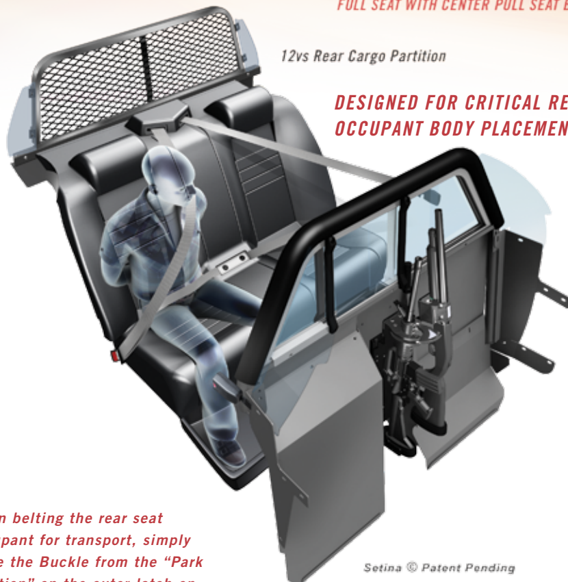
FULL SEAT WITH CENTER PULL SEAT BELTS
